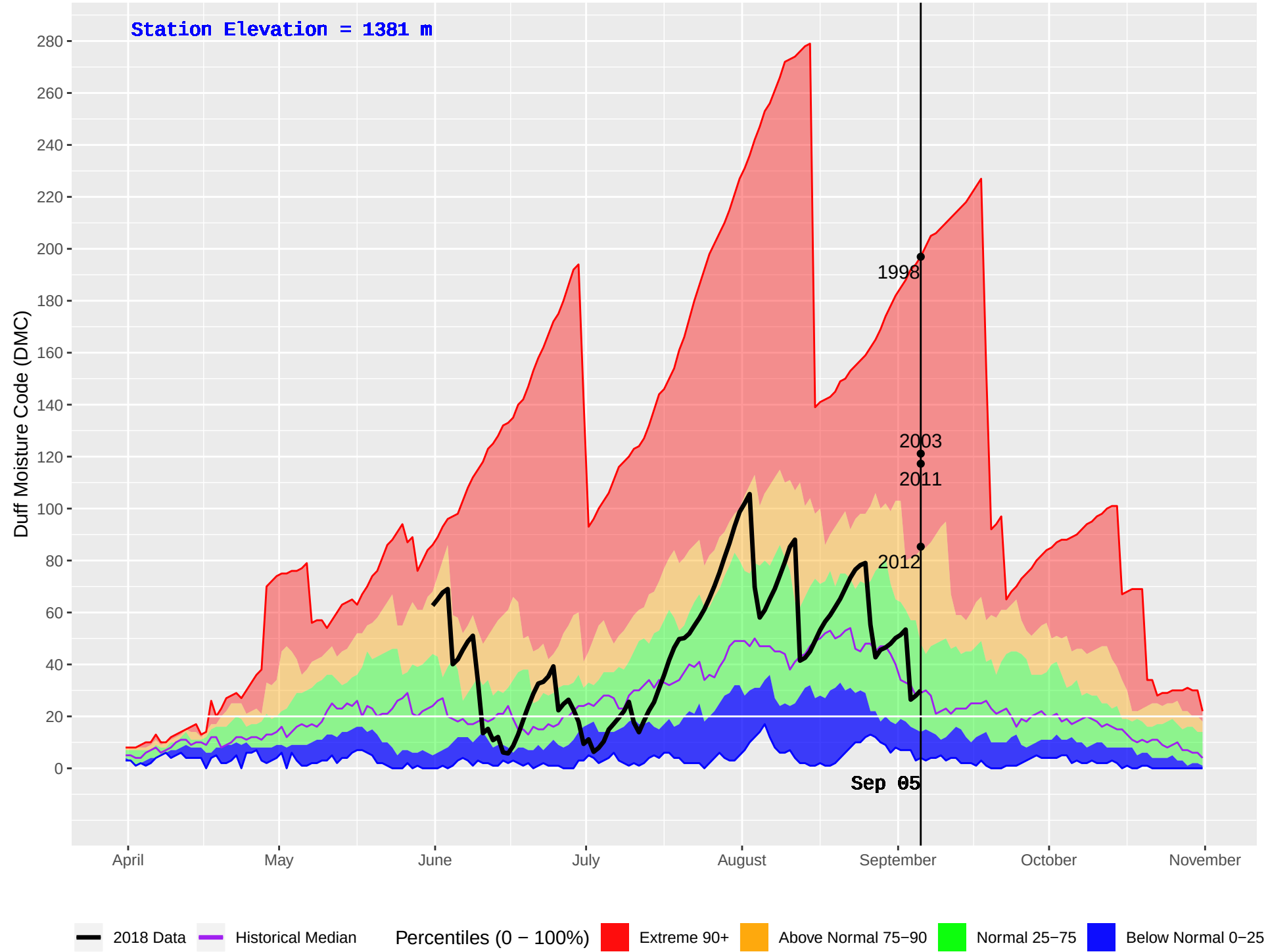
GLIMPSE (291) : Historical (1978–2016) and Current (2018) Daily Duff Moisture Code (DMC)
