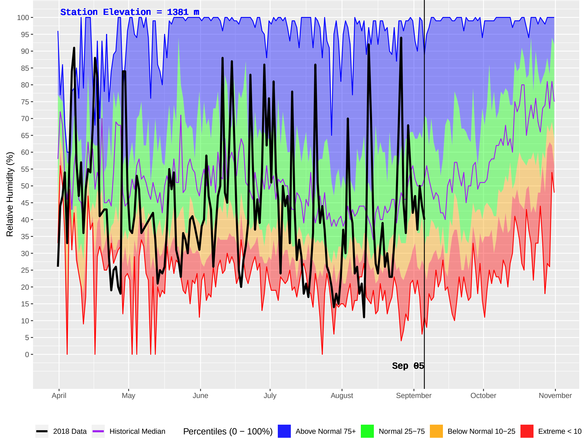
GLIMPSE (291) : Historical (1978–2016) and Current (2018) Daily Relative Humidity
