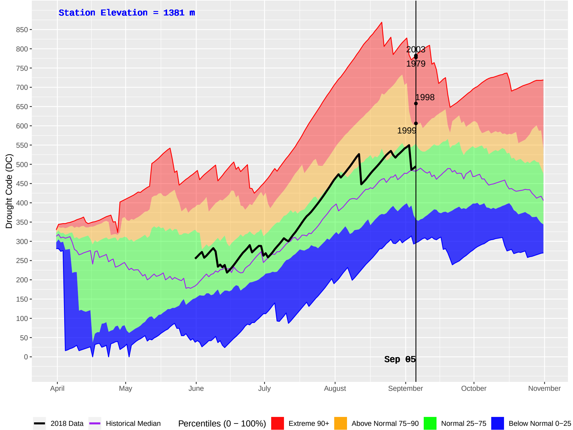
GLIMPSE (291) : Historical (1978–2016) and Current (2018) Daily Drought Code (DC)
