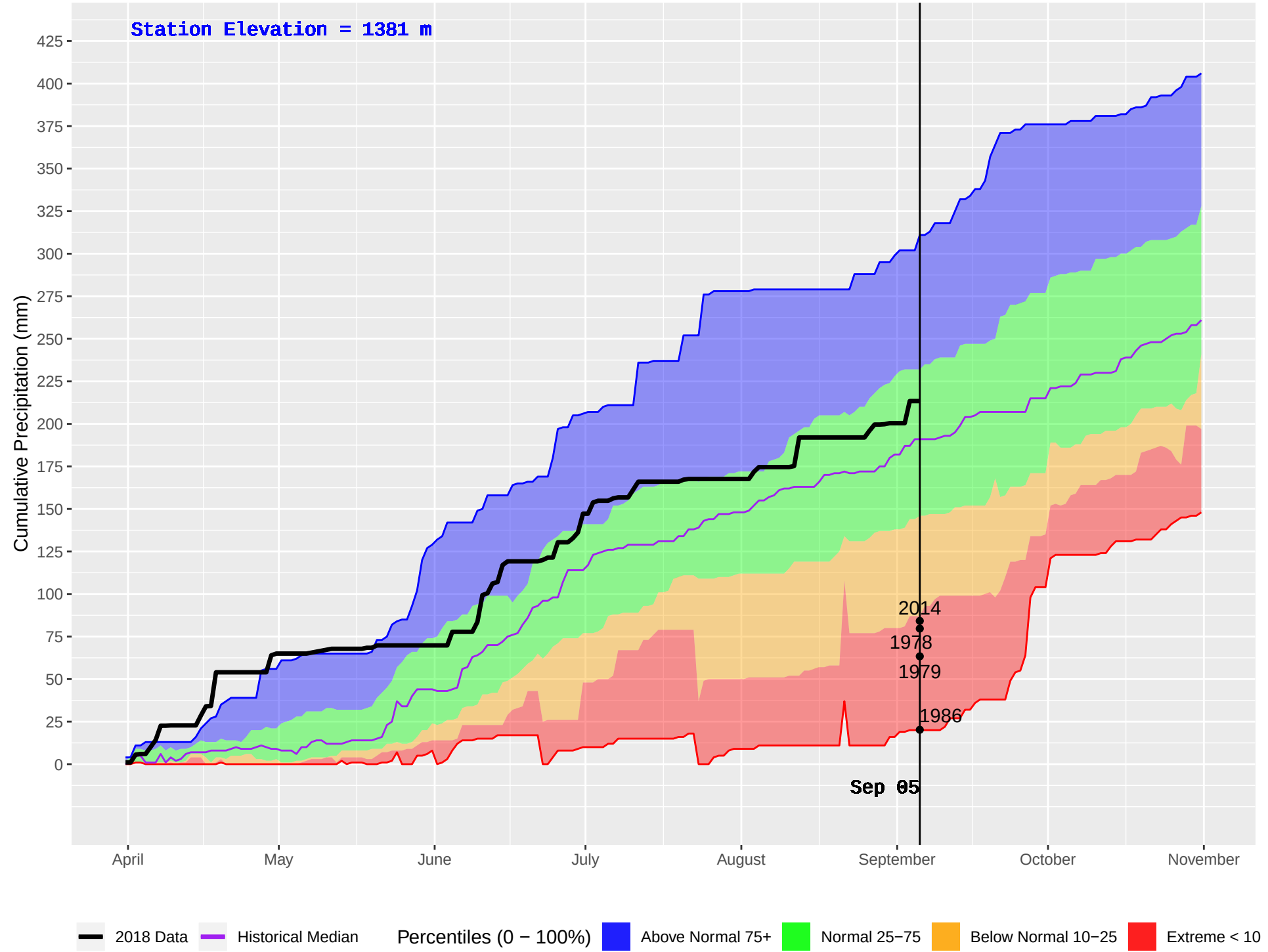
GLIMPSE (291) : Historical (1978–2016) and Current (2018) Daily Cumulative Precipitation
