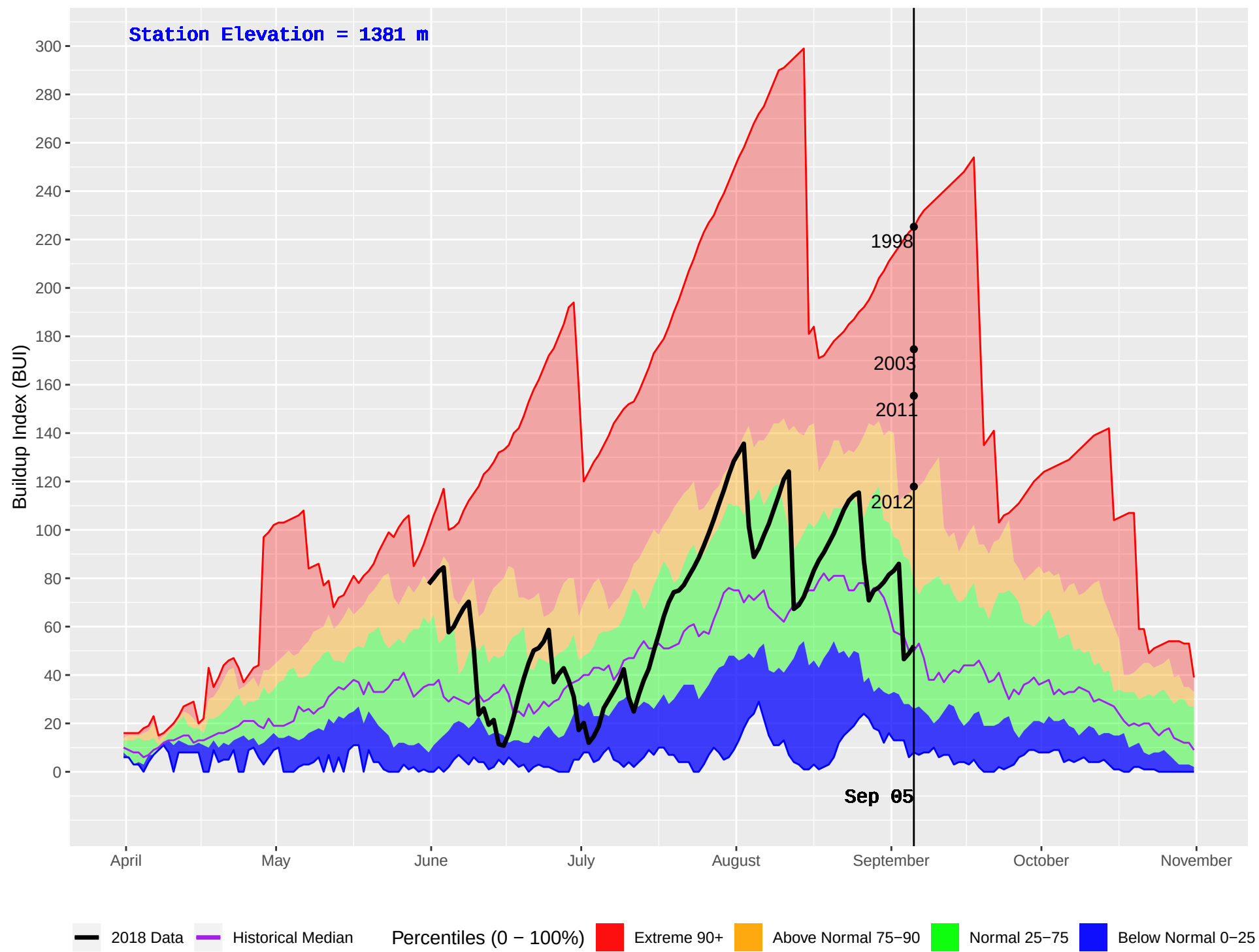
GLIMPSE (291) : Historical (1978–2016) and Current (2018) Daily Buildup Index (BUI)
