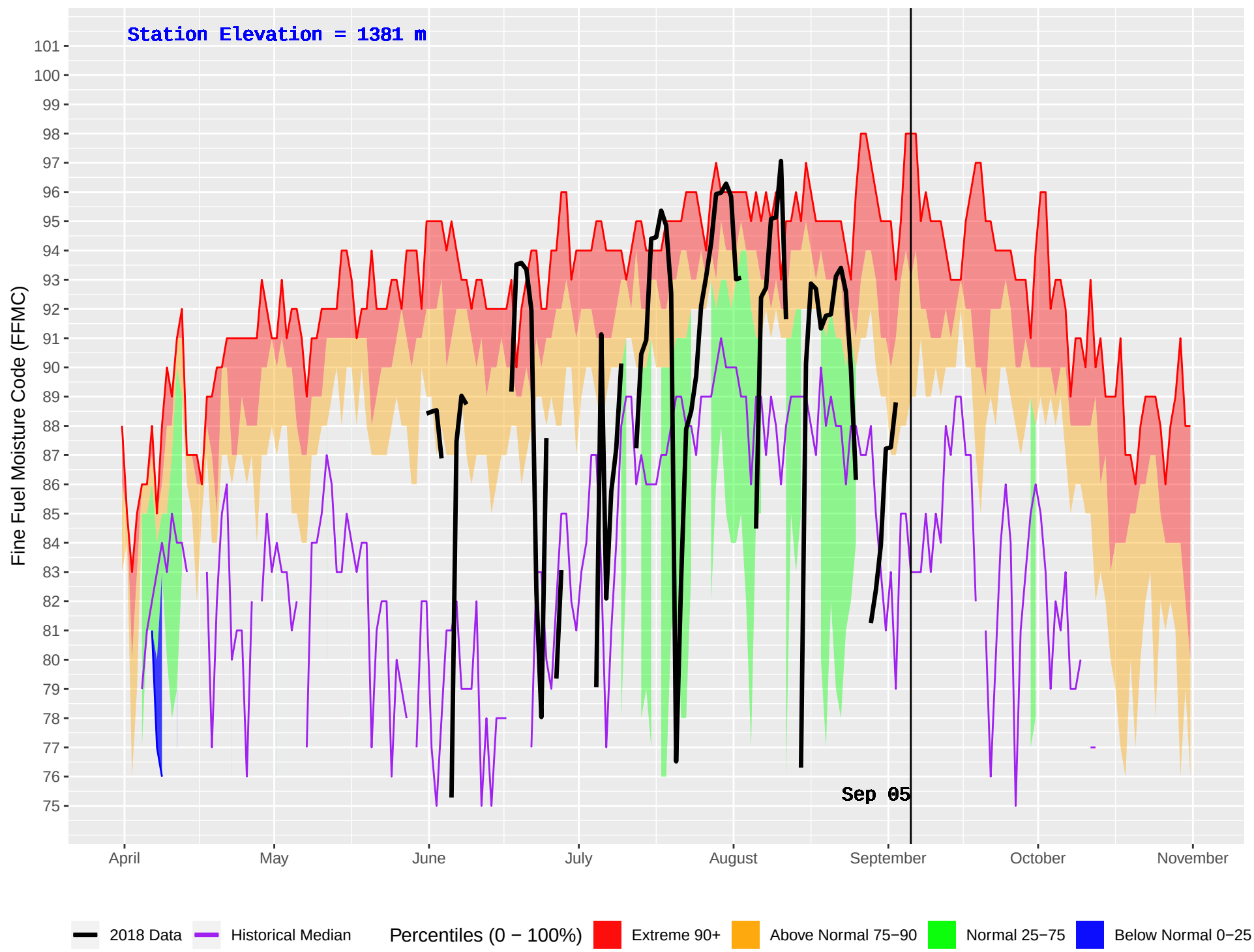
GLIMPSE (291) : Historical (1978–2016) and Current (2018) Daily Fine Fuel Moisture Code (FFMC)
